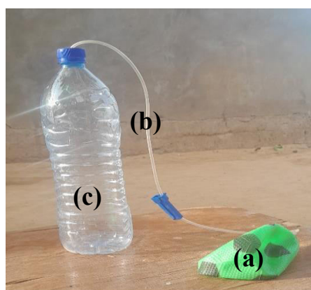
Figure.1 Biodigester
